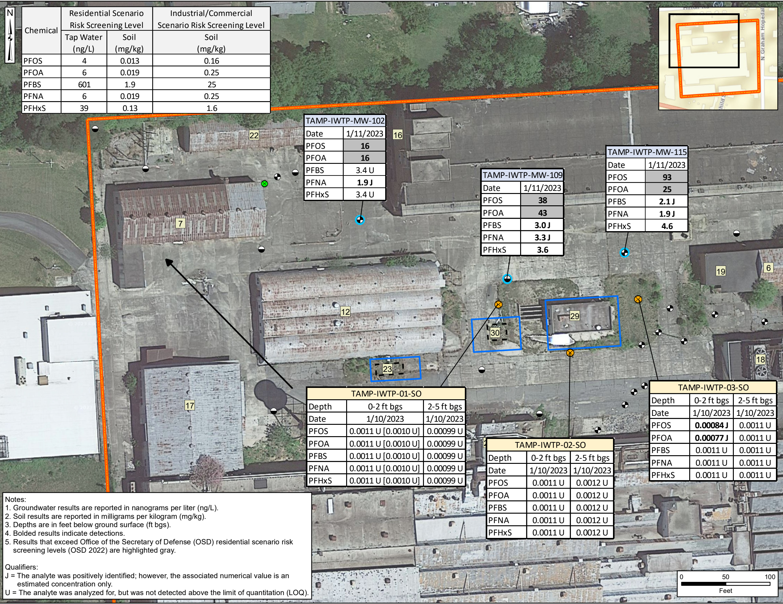
Figure 7-3 IWTW Area (Buildings 23, 29, and 30) PFOS, PFOA, PFBS, PFNA, and PFHxS Analytical Results
